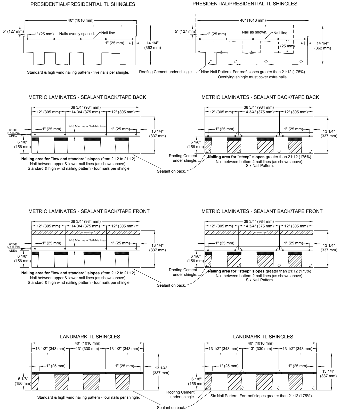
FIGURE 1—SHINGLE PROFILES AND FASTENER PATTERNS (Continued)
