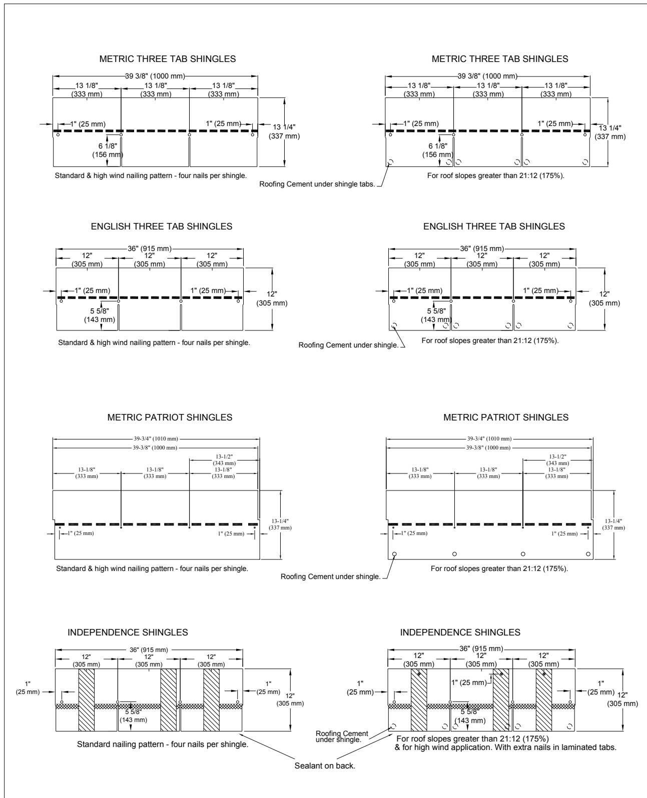
FIGURE 1—SHINGLE PROFILES AND FASTENER PATTERNS
