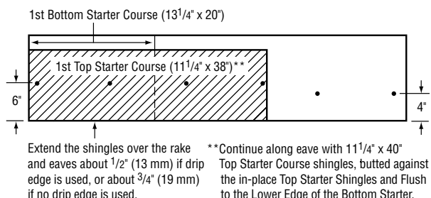
Figure 15-11: Use two (2) overlapping layers of CertainTeed's "Presidential Starter."
