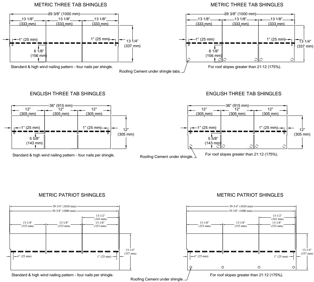
FIGURE 1—SHINGLE PROFILES AND FASTENER PATTERNS
