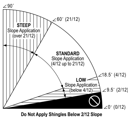
Figure 10-1: Slope definitions.
