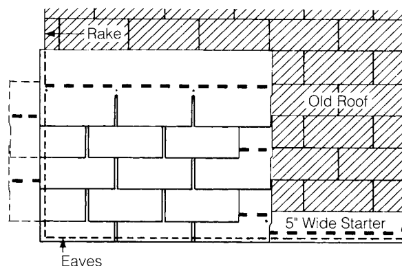
Figure 10-22: Vertical Racking, Nested.
