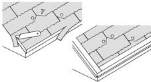
Figure 10-19: Preparing an old roof for reroofing.
