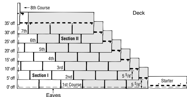
Figure 10-15: Eight-Course, Five-Inch, Stepped-Off Diagonal Method.
