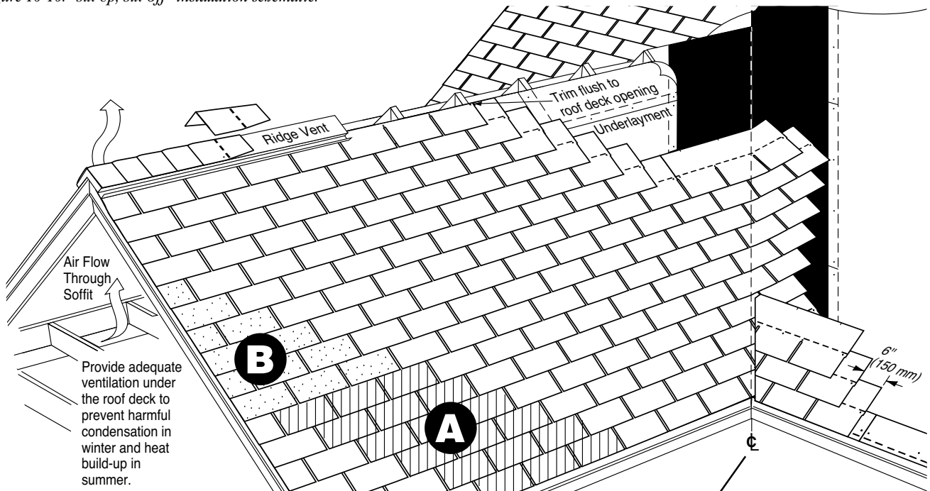
Figure 10-10: "Six Up, Six Off" installation schematic.
