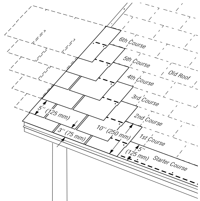
Figure 10-20: Six Off, Six Up, Nested.
