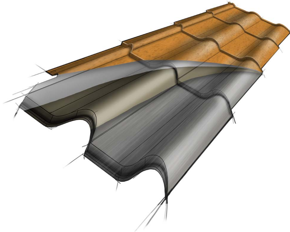
FIGURE 1 –SPANISH TILE PROFILE DETAIL
