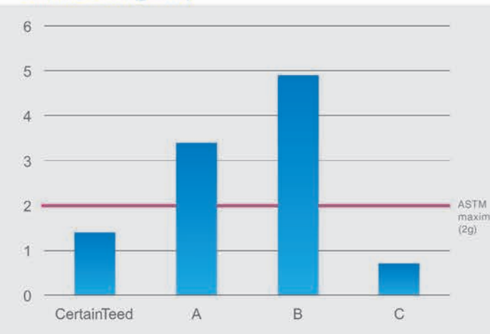
GRAPH D Granule Loss (grams)
