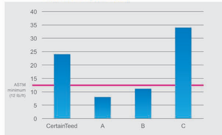
GRAPH A Adhesion to Plywood (lb/ft)
