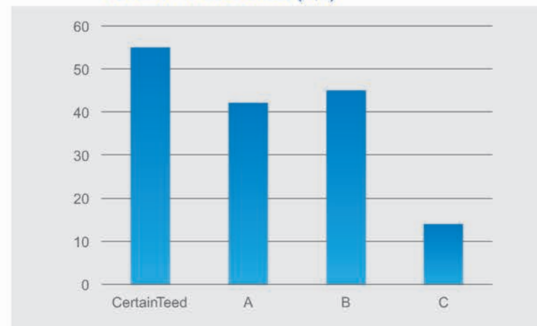
GRAPH B Adhesion to Base Sheet (lb/ft)
