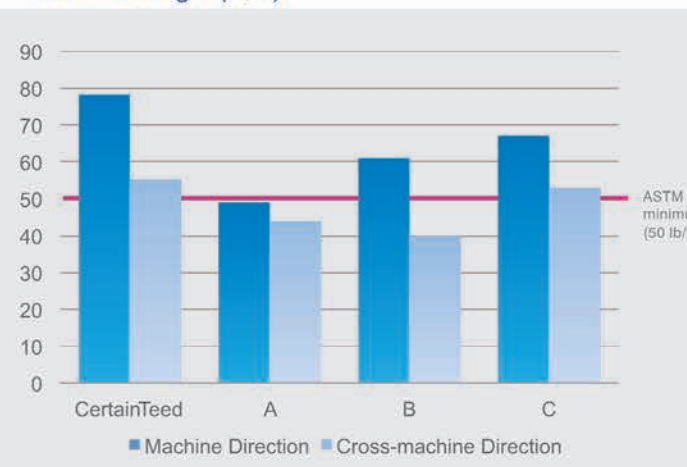
GRAPH E Tensile Strength (lb/in)
