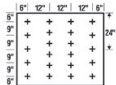
22 Fasteners/Board
