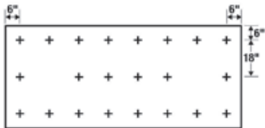
22 Fasteners/Board
