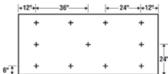
11 Fasteners/Board
