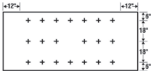
20 Fasteners/Board
