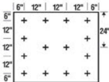
14 Fasteners/Board
