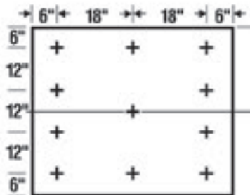
11 Fasteners/Board
