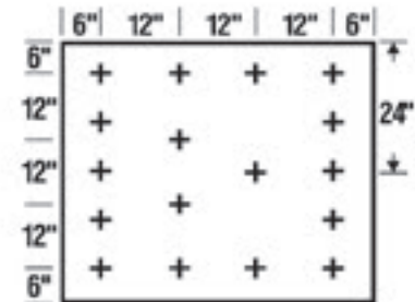
17 Fasteners/Board
