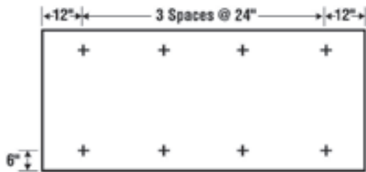
8 Fasteners/Board
