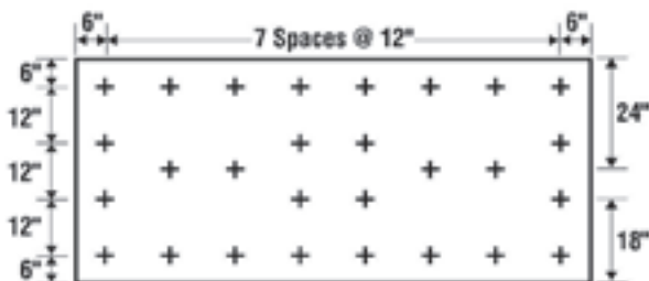
28 Fasteners/Board
