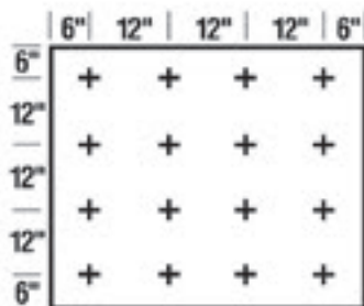
16 Fasteners/Board
