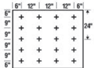
20 Fasteners/Board
