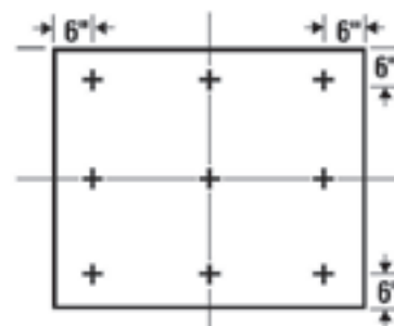
9 Fasteners/Board
