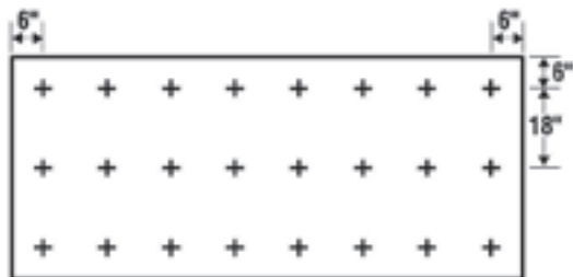
24 Fasteners/Board
