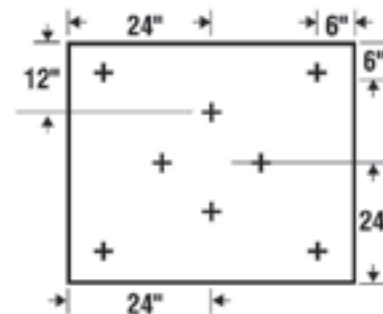
8 Fasteners/Board
