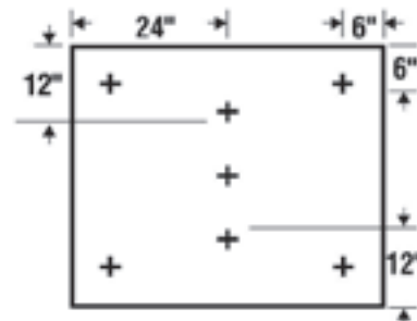
7 Fasteners/Board
