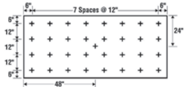
33 Fasteners/Board
