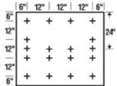
18 Fasteners/Board
