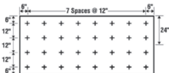
32 Fasteners/Board
