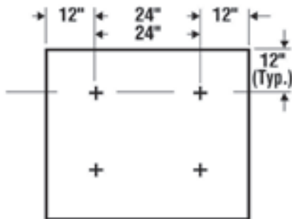
4 Fasteners/Board
