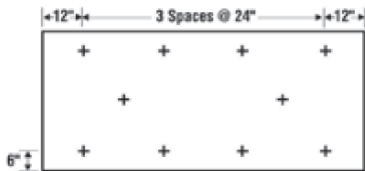
10 Fasteners/Board
