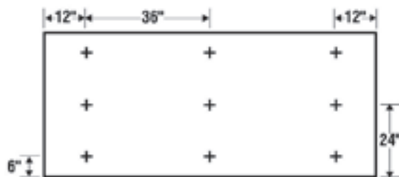
9 Fasteners/Board
