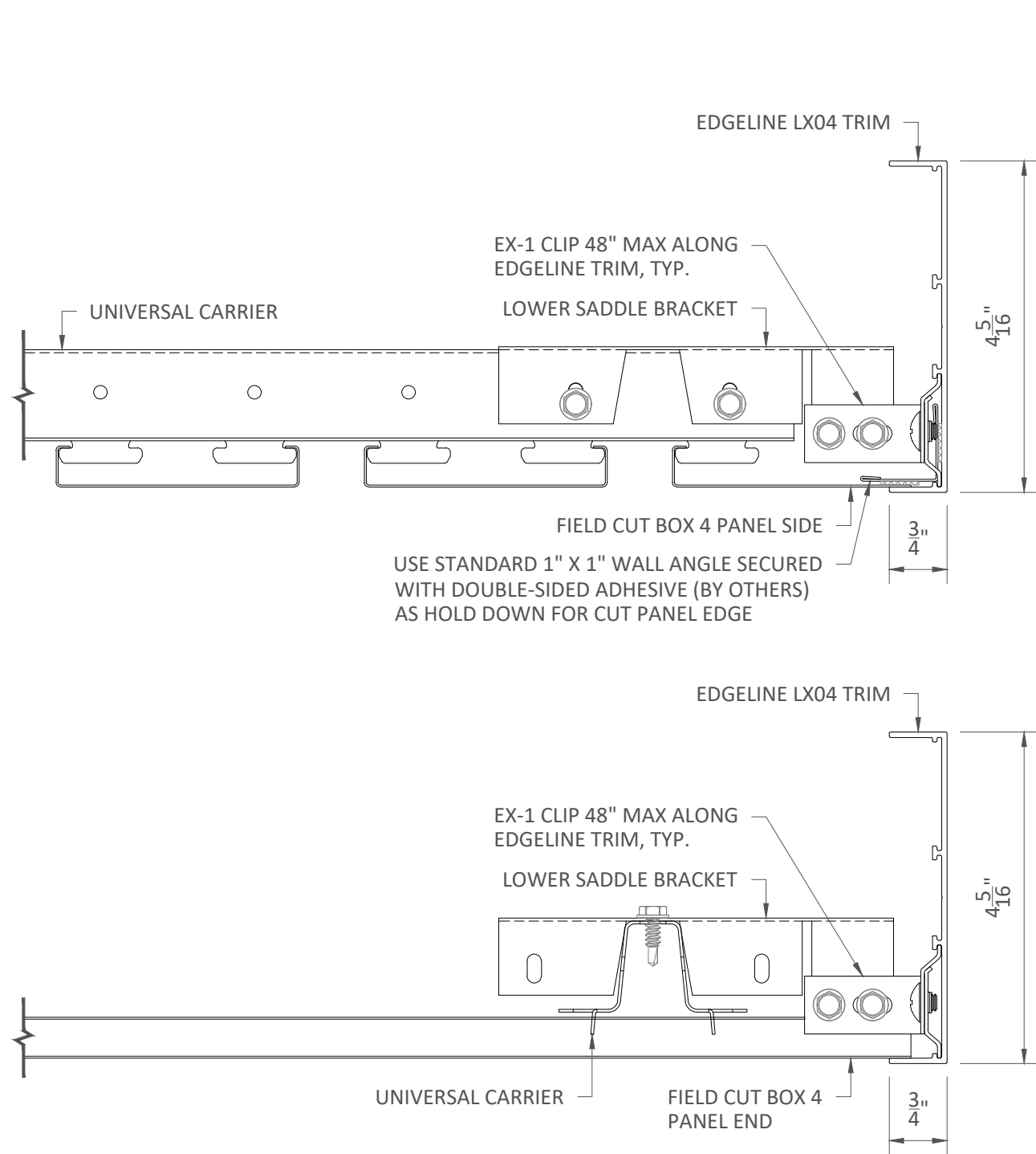
TYPICAL SECTIONS SCALE: 6" = 1'-0"
