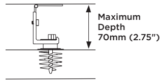
Absorber Bracket Ceiling Application
