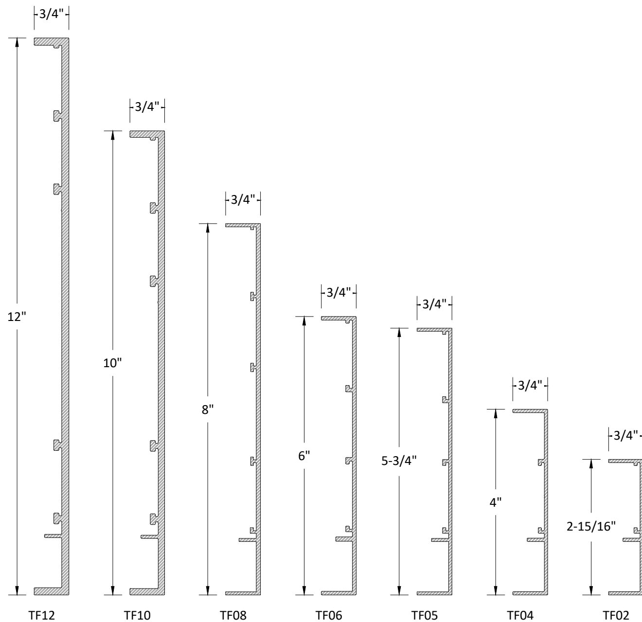
TF EDGELINE PROFILES SCALE: HALF (1:2)
