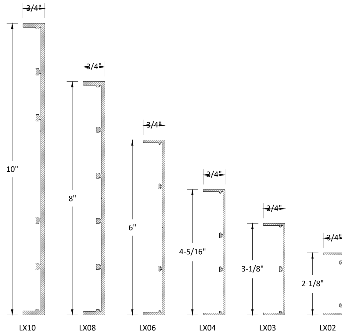
LX EDGELINE PROFILES SCALE: HALF (1:2)
