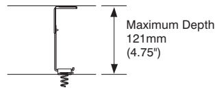
Adjustable Bracket Ceiling Application
