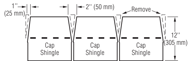
Figure 10-24: Cut tabs, then trim back to make cap shingles (English dimensions shown).
