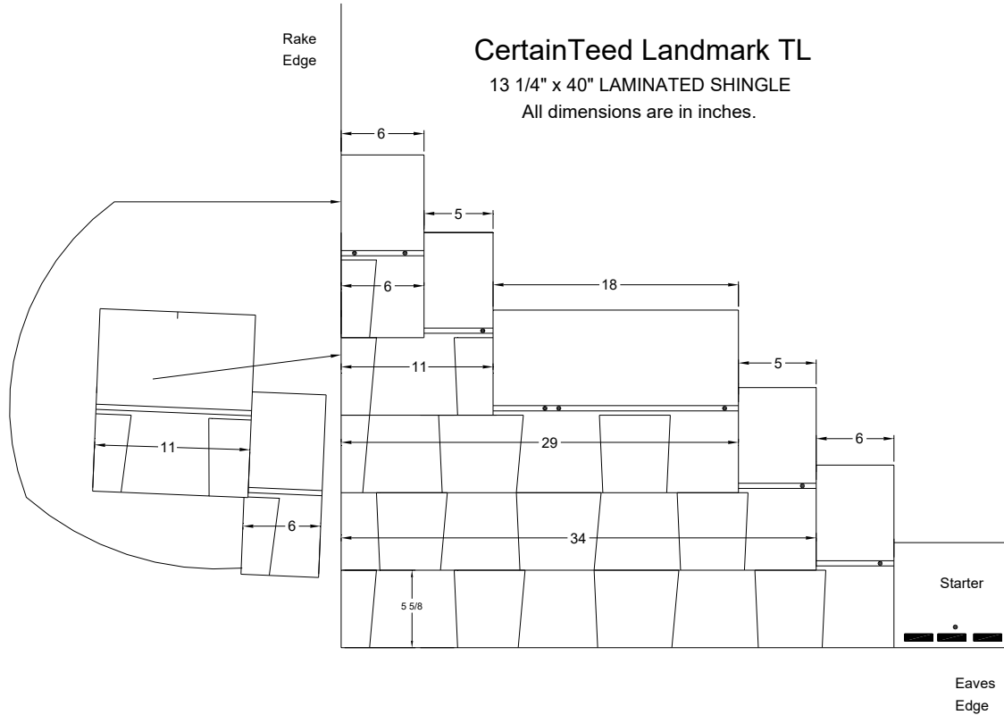
CertainTeed Landmark TL 13 1/4" x 40" LAMINATED SHINGLE All dimensions are in inches.
