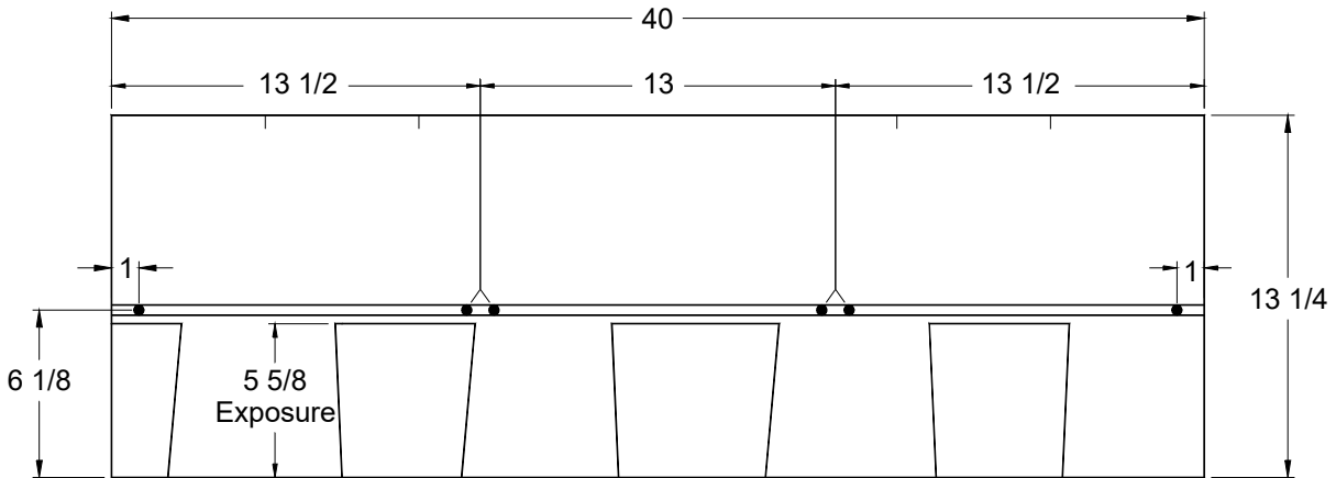
CertainTeed Landmark TL 13 1/4" x 40" LAMINATED SHINGLE All dimensions are in inches.
