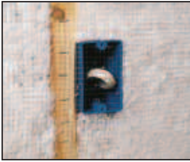
BIBS with InsulSafe SP completely surrounds electrical boxes to help prevent costly drafts and cold spots.
